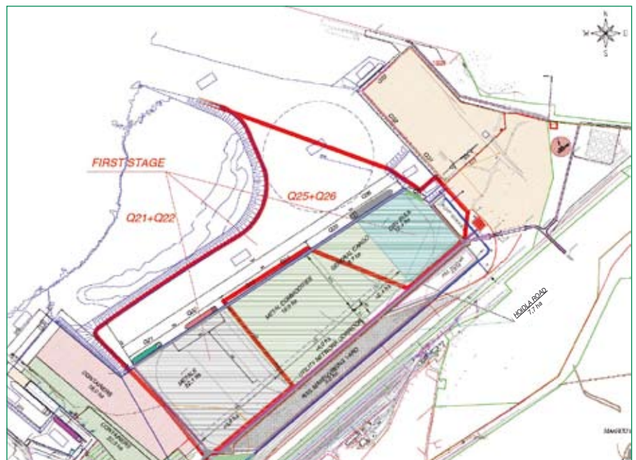
Figure 3: Layout Alternative 1
